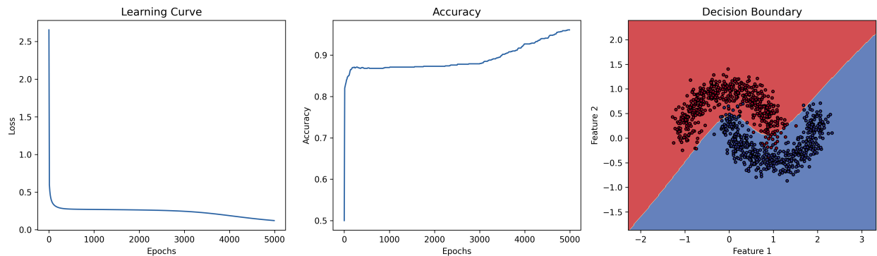
Figure 3: Moons dataset — the network carves a smooth nonlinear boundary between the two crescents. Architecture: [2, 64, 64, 1], 5000 epochs.
