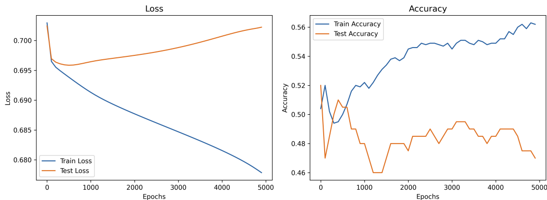
Figure 7: Cats vs dogs — train loss keeps falling, but test accuracy stays flat. Classic overfitting.
