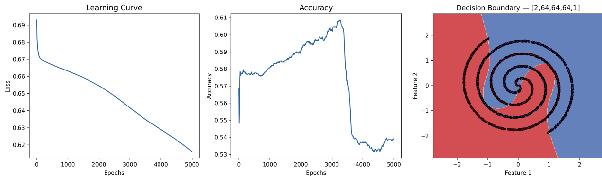
Figure 5: Spirals with 3 hidden layers [2, 64, 64, 64, 1] — the boundary starts wrapping around the spiral arms.
