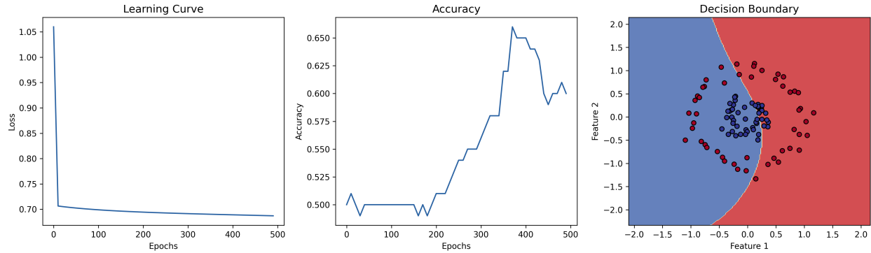
Figure 2: Circles dataset — learning curve, accuracy, and decision boundary. Architecture: [2, 32, 32, 1], 500 epochs.
